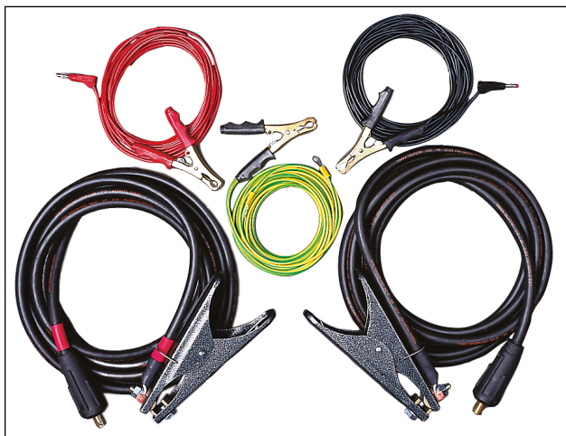
Cable set standard GA-05055 (current cables and sensing cables) and ground cable GA-00200.
