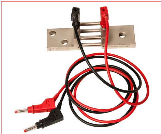
Current shunt for calibration, BB-90024
