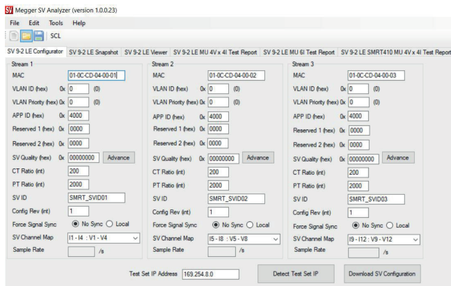
Figure 6: Megger Sampled Values Configurator
