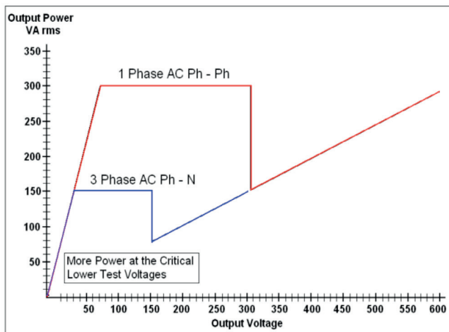
Figure 4: Voltage output power curve
