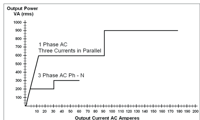
Figure 3: Current output power curve
