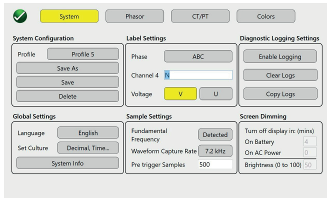
Figure 2: Configuration screen
