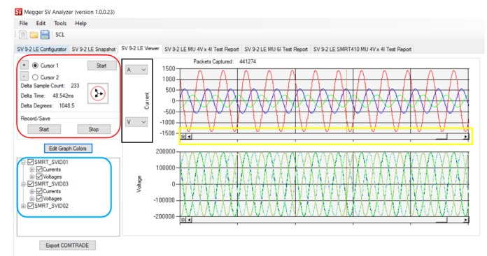
Figure 17: SV Viewer
