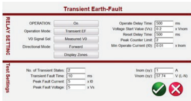
Figure 19: Transient Earth Fault Test Setting Screen
