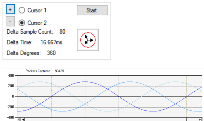
Figure 18: Snipped waveform on "SV Viewer" tab
