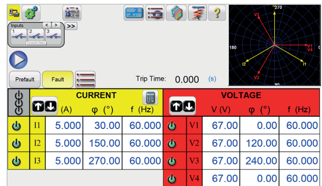
Figure 2: STVI advanced user interface
