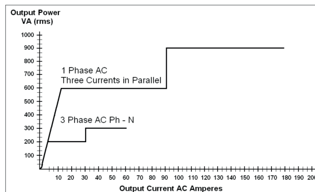
Figure 3: Current output power curve
