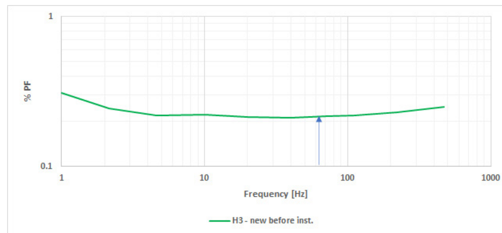
Figure 2: Pre-installation NB DFR test results for H3 replacement bushing
