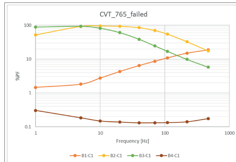
Figure 3: NB DFR plot of failed CVT 1's C1 sections B1 to B4
